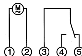
MIL/1 internal schematic
