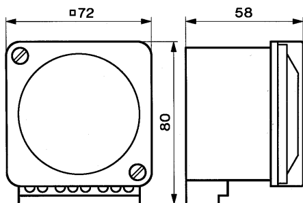
MIL/1 dimensions – dimension over ter-
