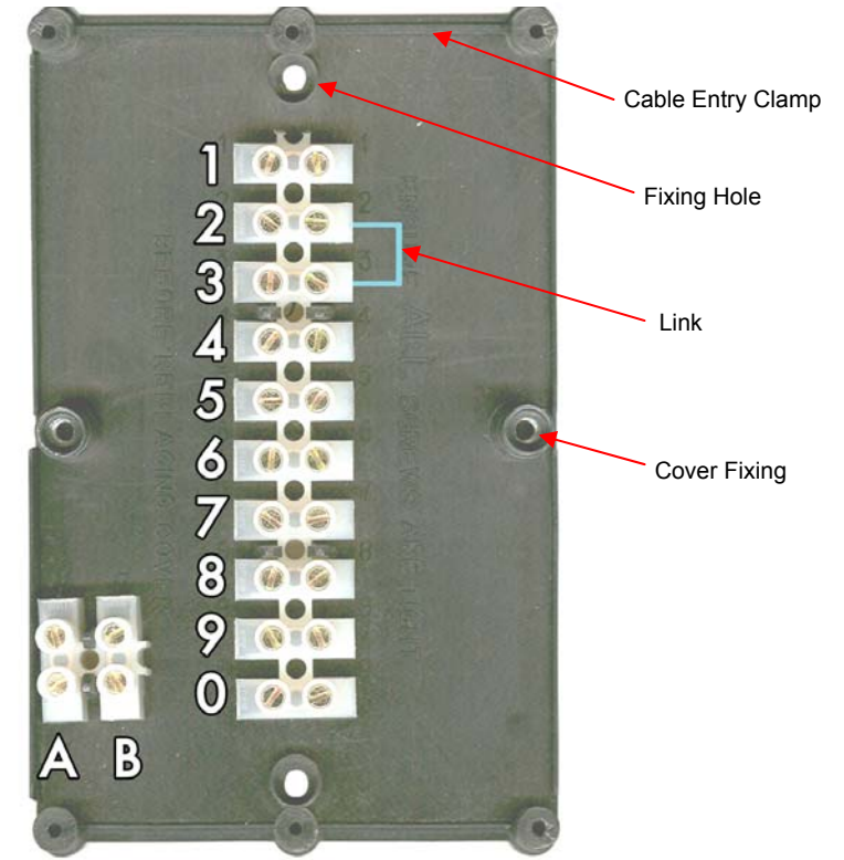
FIGURE. 1 JUNCTION BOX
