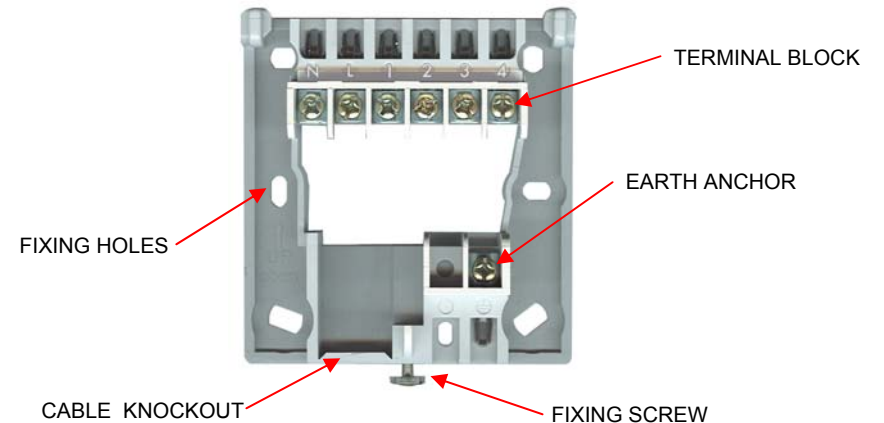
FIGURE. 2 QE2 BASEPLATE
