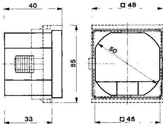
Taxxo 102 – dimensional details
